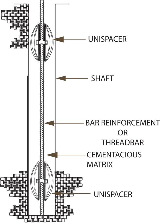
SHAFT ELEVATION NO SCALE
